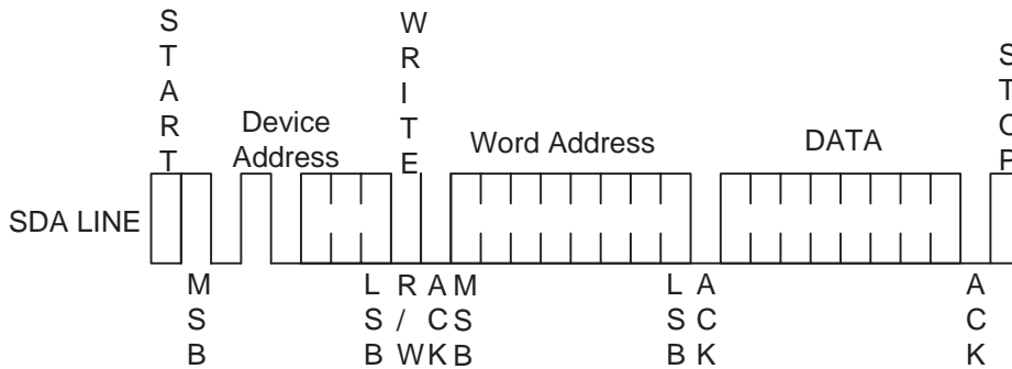
Figure 3: Byte Write
