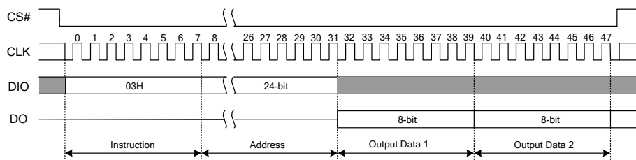
Figure 7.5 Read Data Instruction Sequence Diagram
