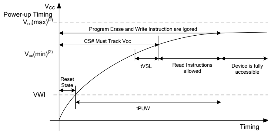
Figure 8.1 Power-up Timing
