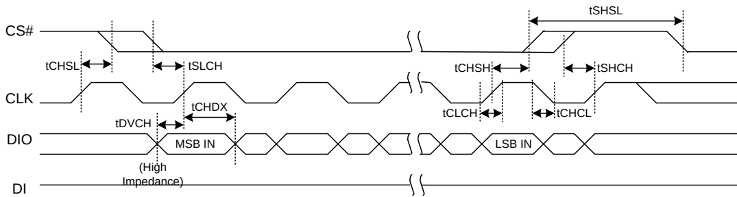
Figure 8.4 Input Timing
