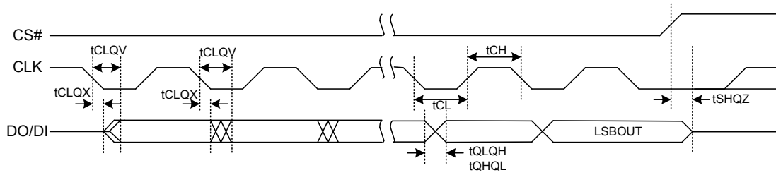
Figure 8.3 Serial Output Timing
