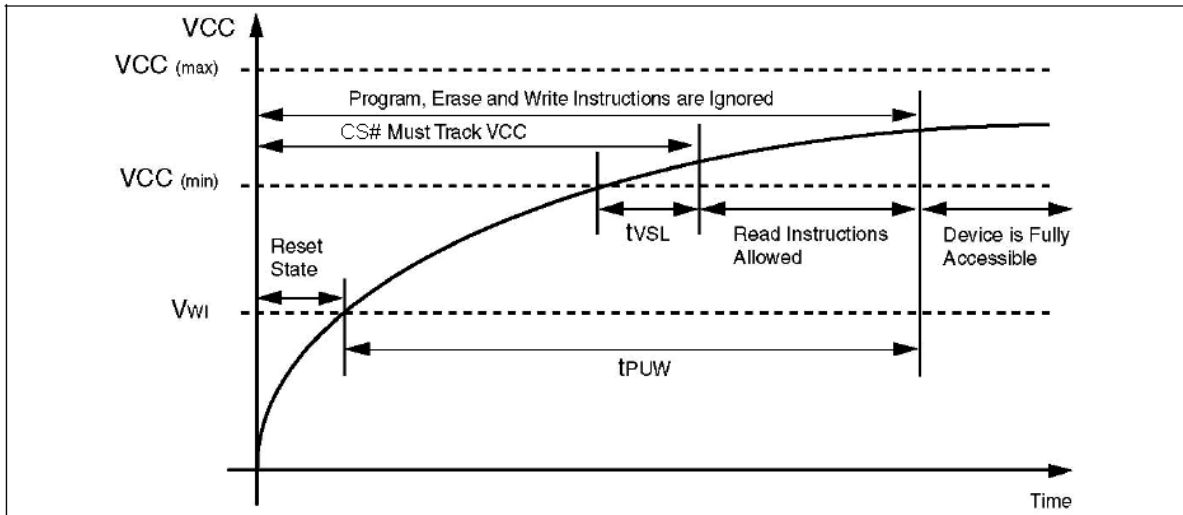
Figure 31. Power-up Timing
