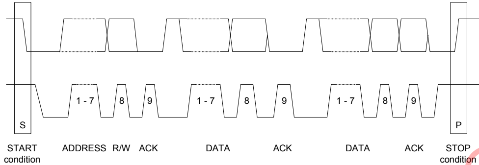
Figure8. I2C Complete Data Transfer
